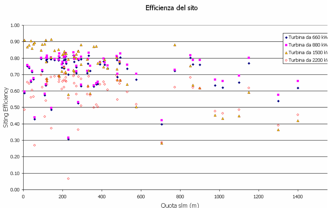
Fig. 4.13 – Siting Efficiency dell’impianto
